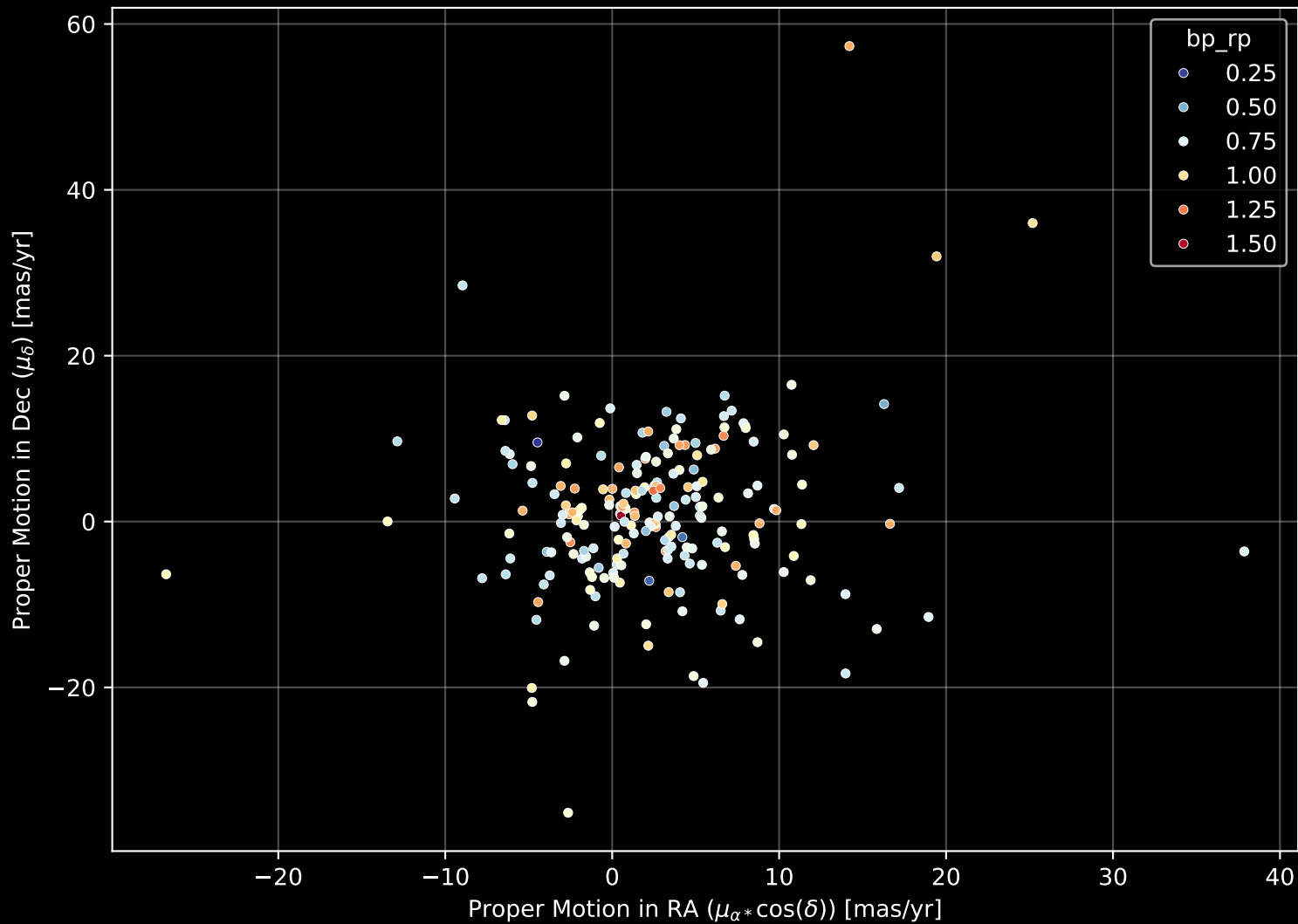
GALAH DR4 Field: [625] Proper Motion Diagram (n= 209)
